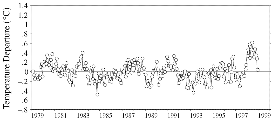
Figure 3 Satellite-Measured Temperatures for the Southern Hemisphere
