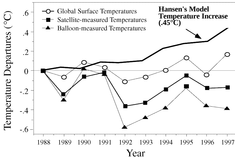
Figure 2 Temperature Projections and Observations: 1988-97
