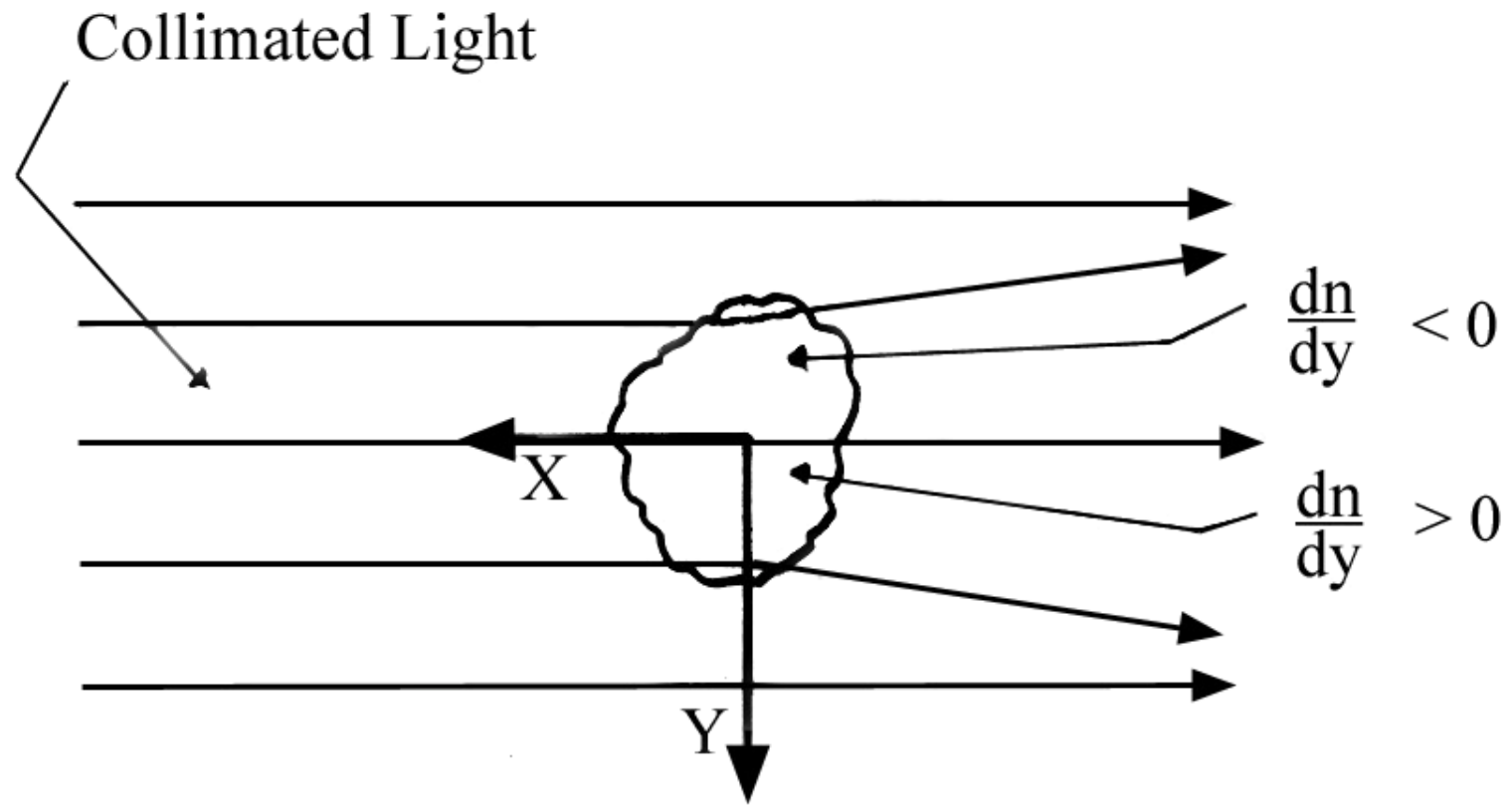
Figure 1. Disturbance in Collimated Beam
