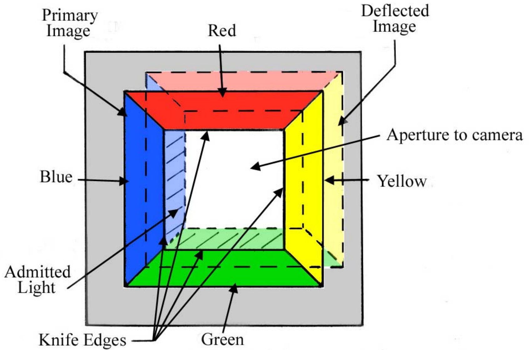
Figure 6. Filter Image on Knife Edges
