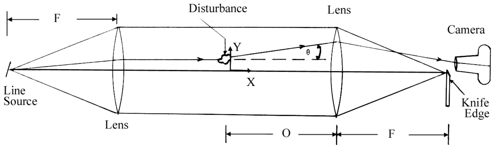
Figure 3. Schlieren System with a Small Disturbance
